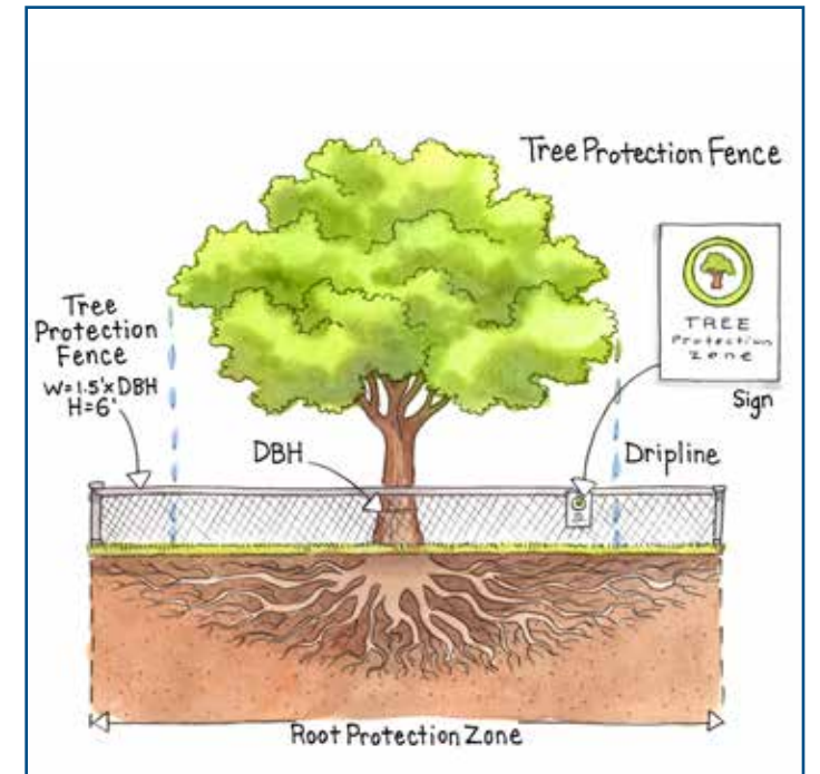
Tree Protection Fence and Signage
